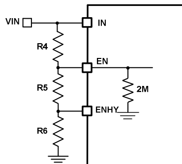
Figure 6 – Adjustable UVLO using EN &amp; ENHY pin
