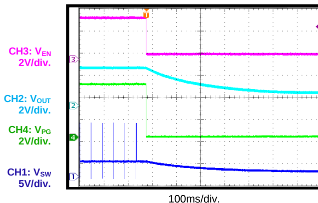
Low-Dropout Mode
