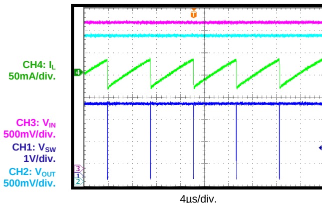
Low-Dropout Mode
