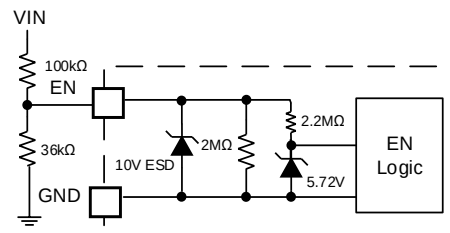
Figure 8: EN Internal Circuit
