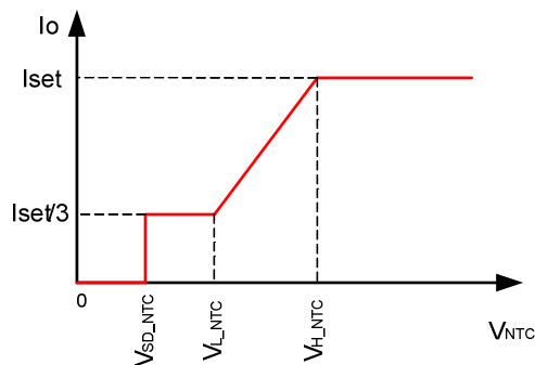
Figure 19: NTC Curve
