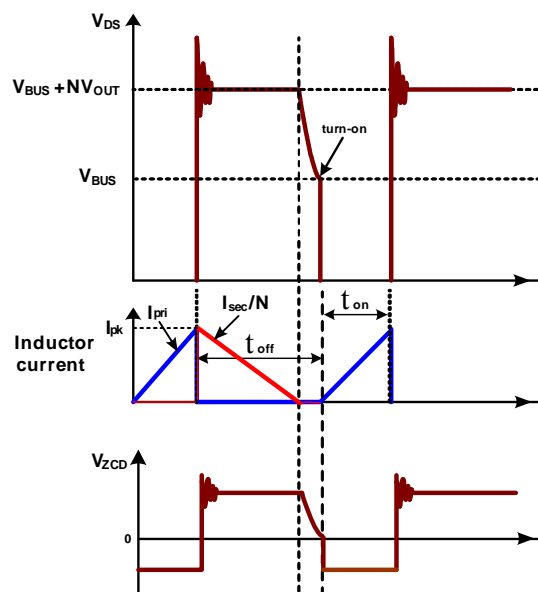
Figure 3: Boundary-Conduction Mode
