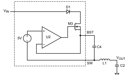
Figure 3—Internal Bootstrap Charging Circuit Startup and Shutdown
