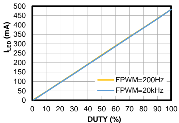
PWM Dimming
