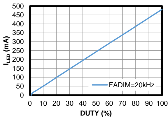
Analog Dimming
