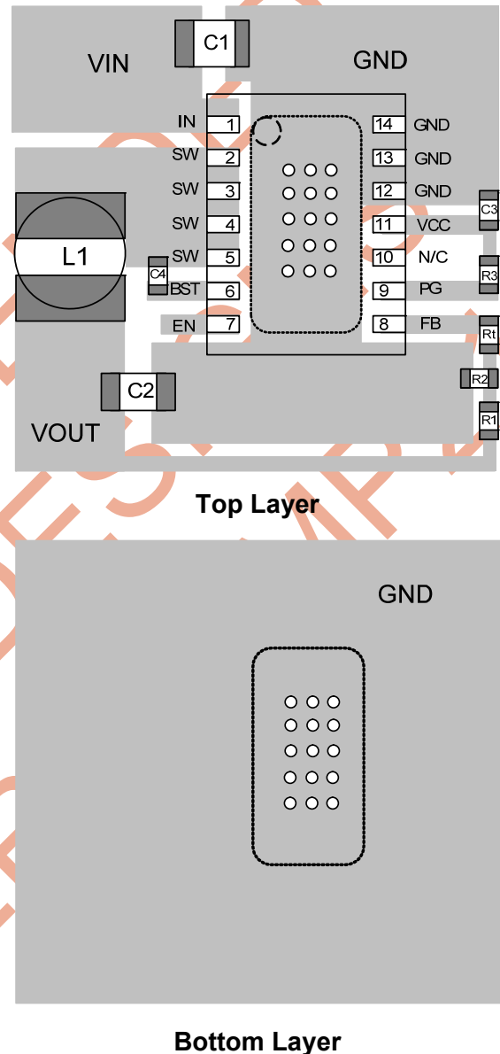
Figure 7—PCB Layout
