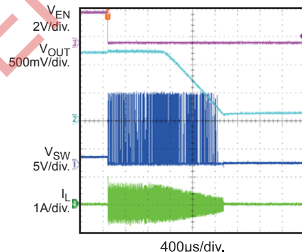
Power down through EN I_{OUT} = 0A
