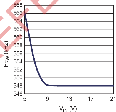
Frequency vs. Input Voltage R_{F_{SW}} = 274k\Omega , I_{OUT} = 4A
