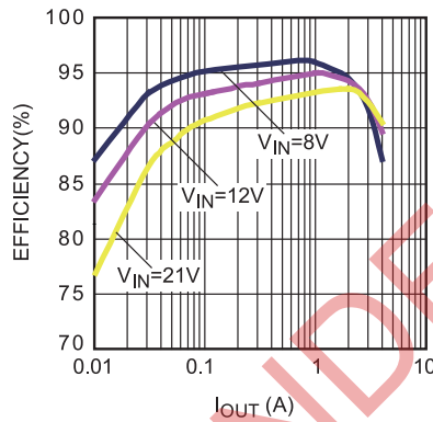
Efficiency vs. Load Current V_{OUT} = 5V , F_{SW} = 550kHz , L = 3.3\mu H
