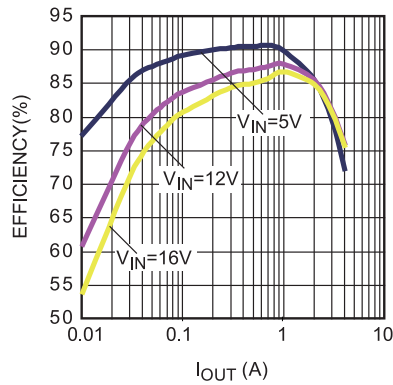
Efficiency vs. Load Current F_{SW} = 500kHz
