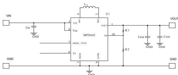
Figure 4—Reference Circuit for PCB Guide
