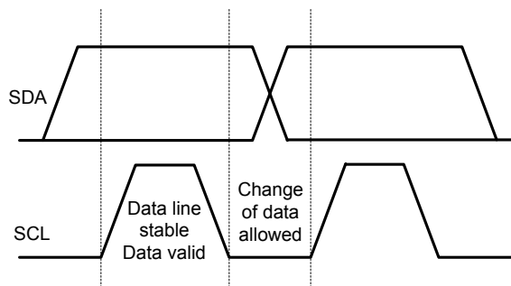
Figure 11: Bit Transfer on the I 2 C Bus
