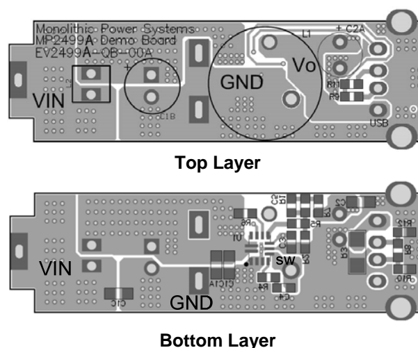
Figure 9: Recommended Layout
