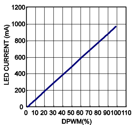
PWM Dimming
