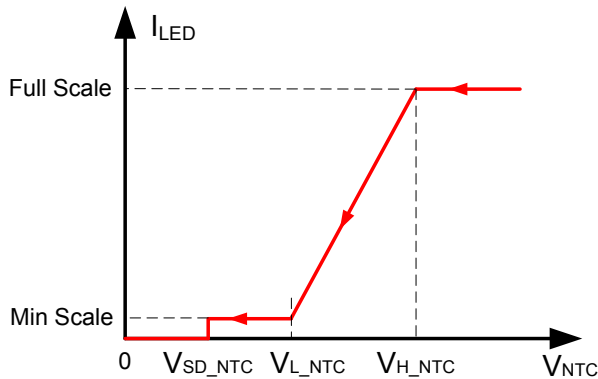
Figure 4: NTC Curve
