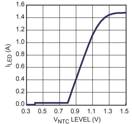
NTC Curve
