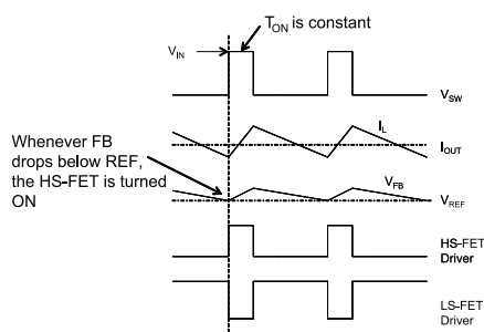
Figure 2: Heavy-Load Operation
