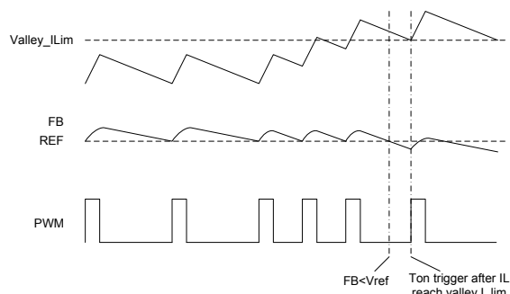
Figure 6: Valley Current-Limit Control
