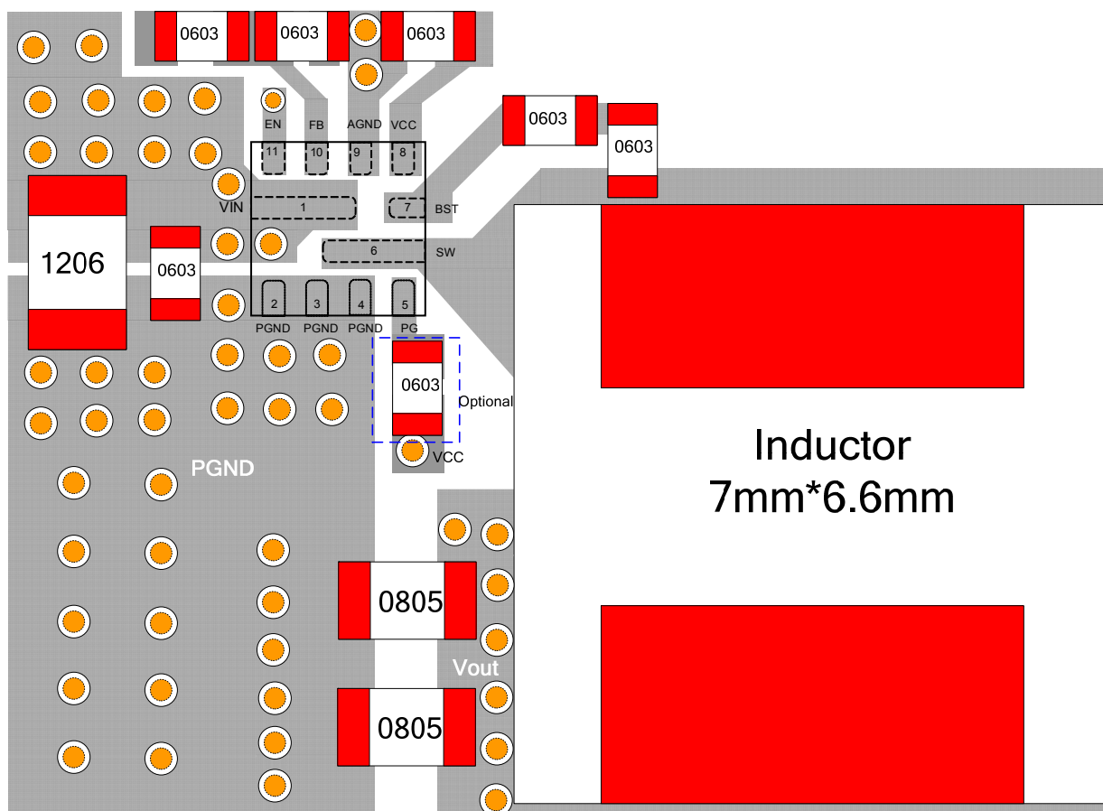
Figure 10: Recommended Layout
