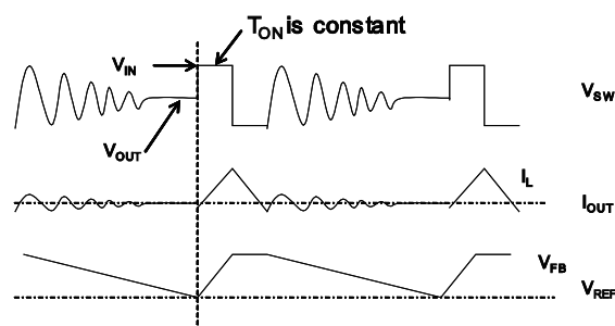
Figure 3: Light-Load Operation
