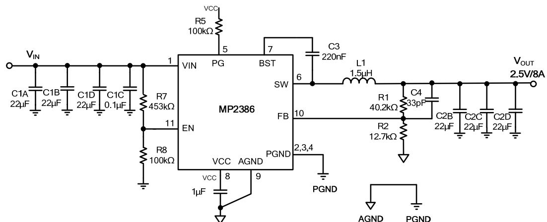
Figure 13: V_{IN} = 19V , V_{OUT} = 2.5V/8A
