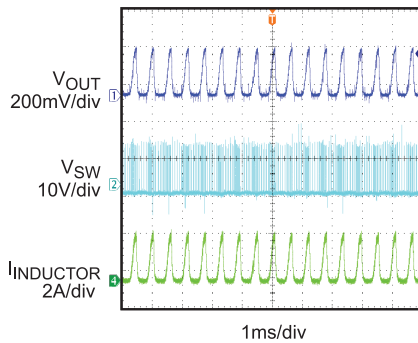
Hiccup with Output Short Circuit
