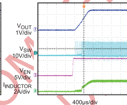
Enable Startup Full Load
