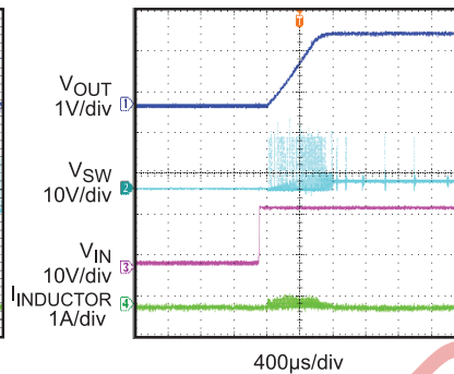
Power Up No Load
