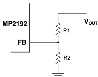
Figure 9: Feedback Network
