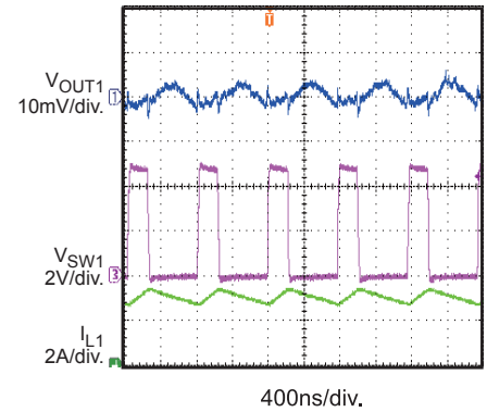
Output Ripple
