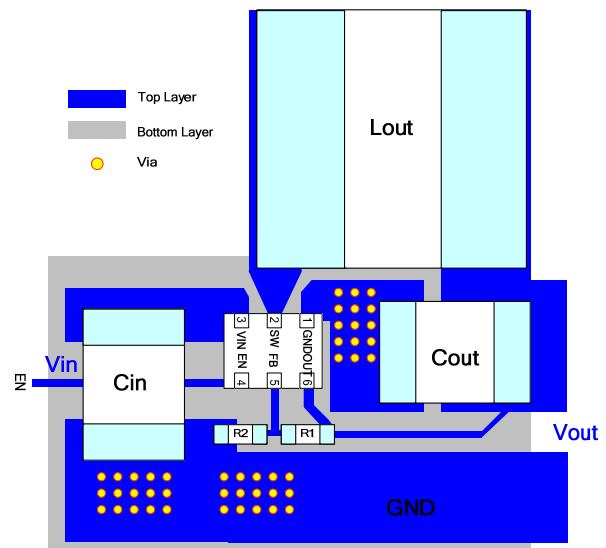
Figure 10: Recommended Layout for the MP2172C
