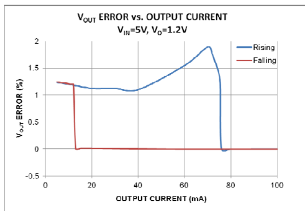
Figure 4: Sleep/DCM Transition @ V_{IN}=5V , V_{OUT}=1.2V
