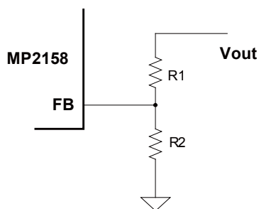
Figure 5: Feedback Network
