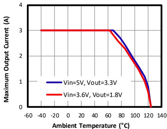
Output Current Derating vs. Ambient Temperature T J ≤ 125°C
