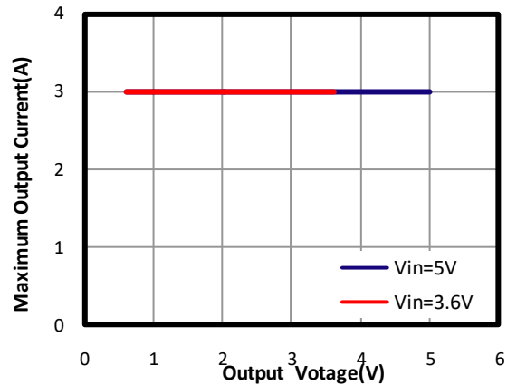
Output Current Derating vs. Output Voltage T J ≤ 125°C
