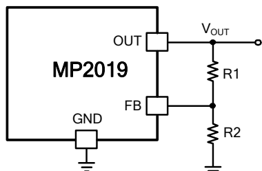
Figure 3. FB Resistor Divider to Set V_{OUT}
