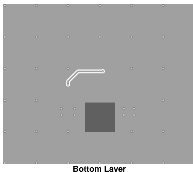
Figure 4: Recommended Layout
