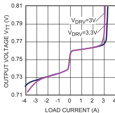
DDR3 Regulation
