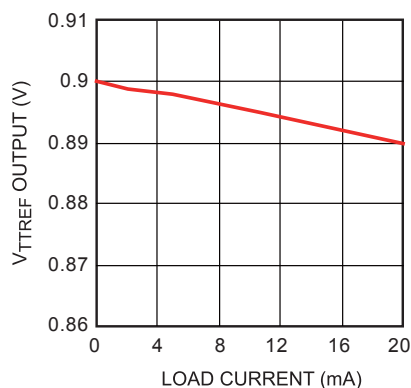
V_{\text{TTREF}} Regulation
