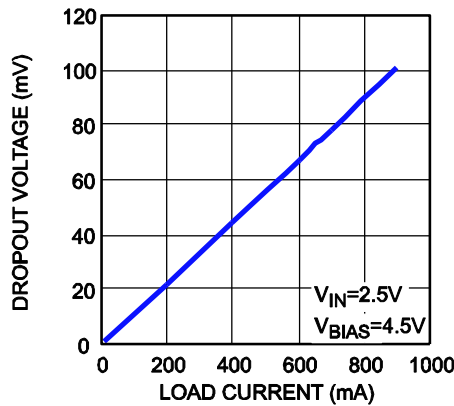
Voltage Dropout
