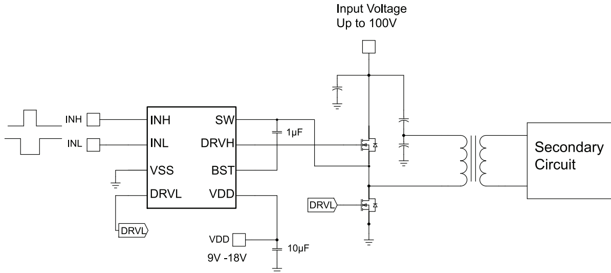
Figure 4: Half-Bridge Converter
