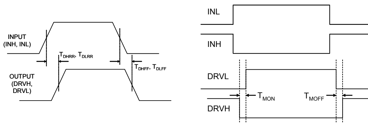
Figure 1: Timing Diagram
