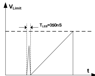
Figure 6: Leading-Edge Blanking
