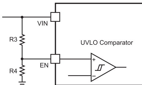
Figure 3: Adjustable UVLO
