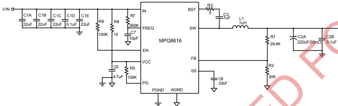
Figure 13 — Typical Application Circuit with No External Ramp
