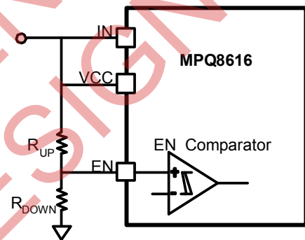
Figure 7—Adjustable UVLO
