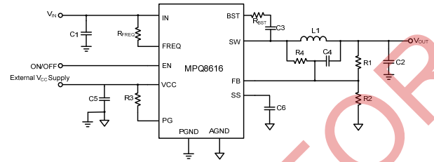
Schematic for PCB Layout Guide Line
