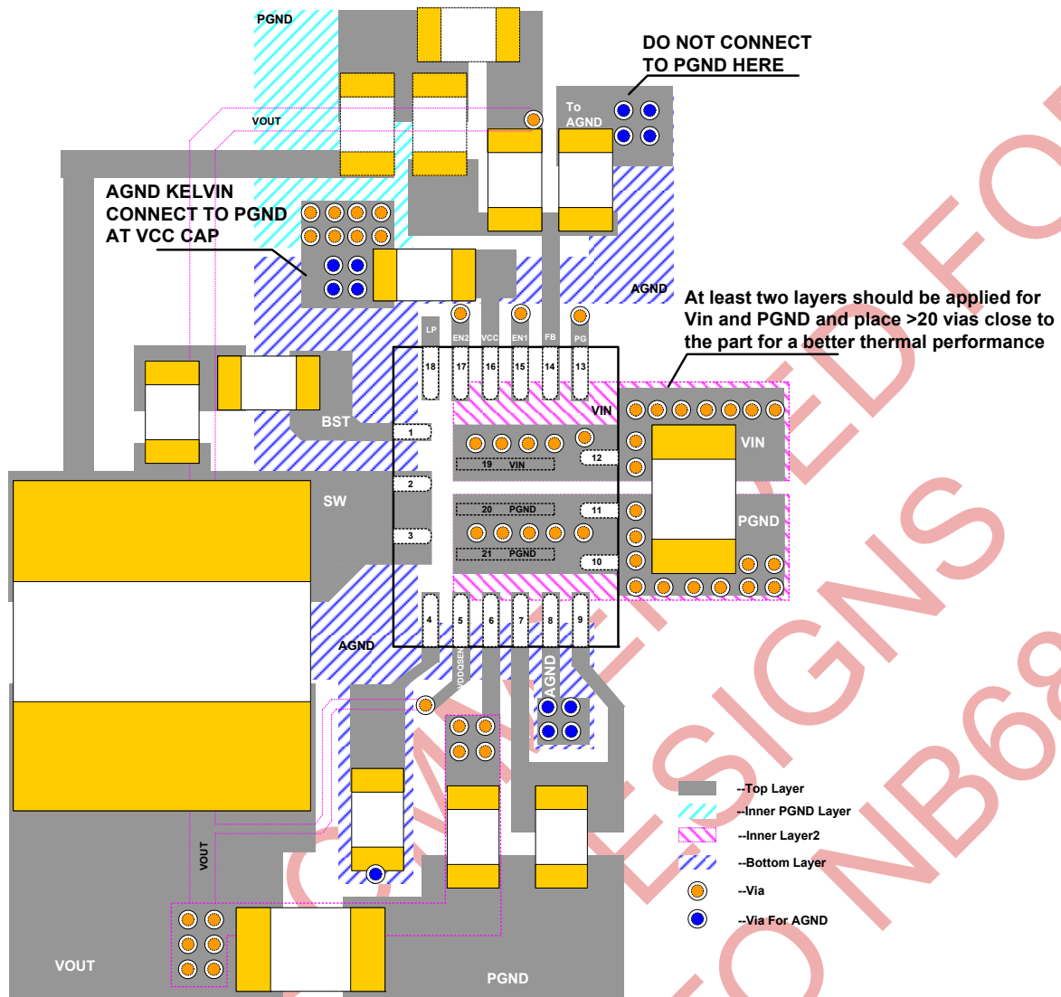
Figure 13—Recommend Layout
