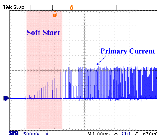
Figure 4—Soft Start
