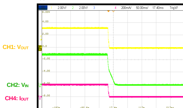
Shutdown through V_{IN} I_{OUT} = 0.2A
