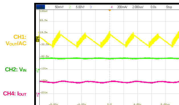
V_{OUT} Ripple I_{OUT} = 0.2A
