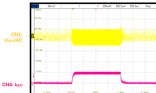
Load Transient I_{OUT} = 0A to 0.2A
