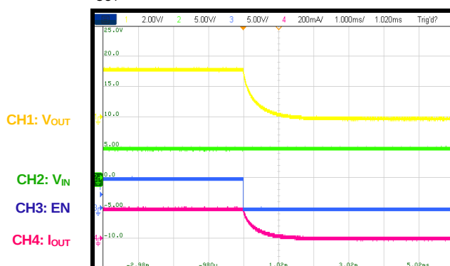
Shutdown through EN I_{OUT} = 0.2A
