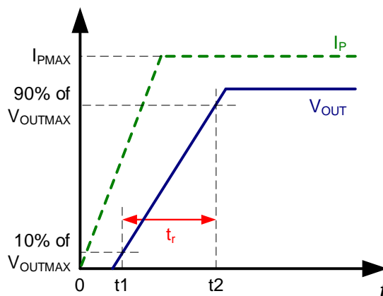
Figure 7: Rise Time ( t_R )
