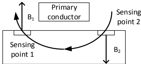
Figure 3: Schematic cross section of the sensor
