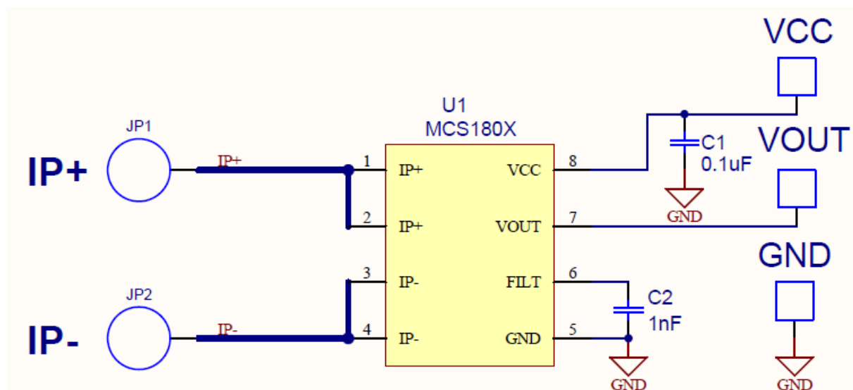
Figure 11: Application Circuit
