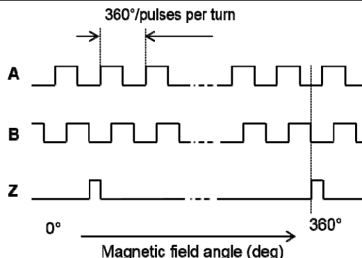
Figure 22: Timing of the ABZ Output
