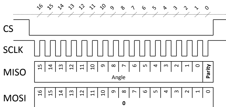
Figure 15: Angle reading with parity bit
