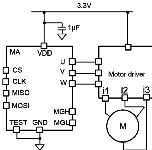
Figure 30: Typical Motor Configuration Using UVW Commutation Signals
