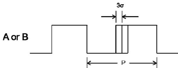
Figure 25: ABZ Jitter
