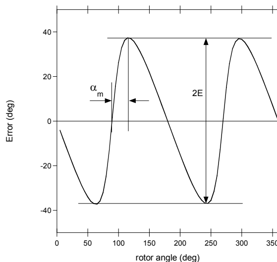
Figure 18: Error Curve in Side-Shaft Configuration with BCT = 0
