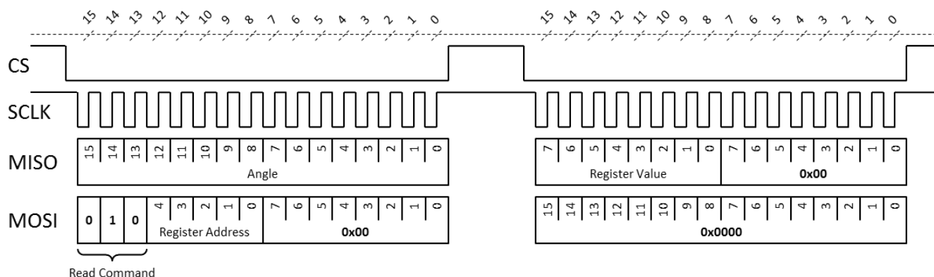
Figure 11: 16-Bit Frames Read Register Operation
