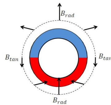
Figure 16: Side-Shaft Field
