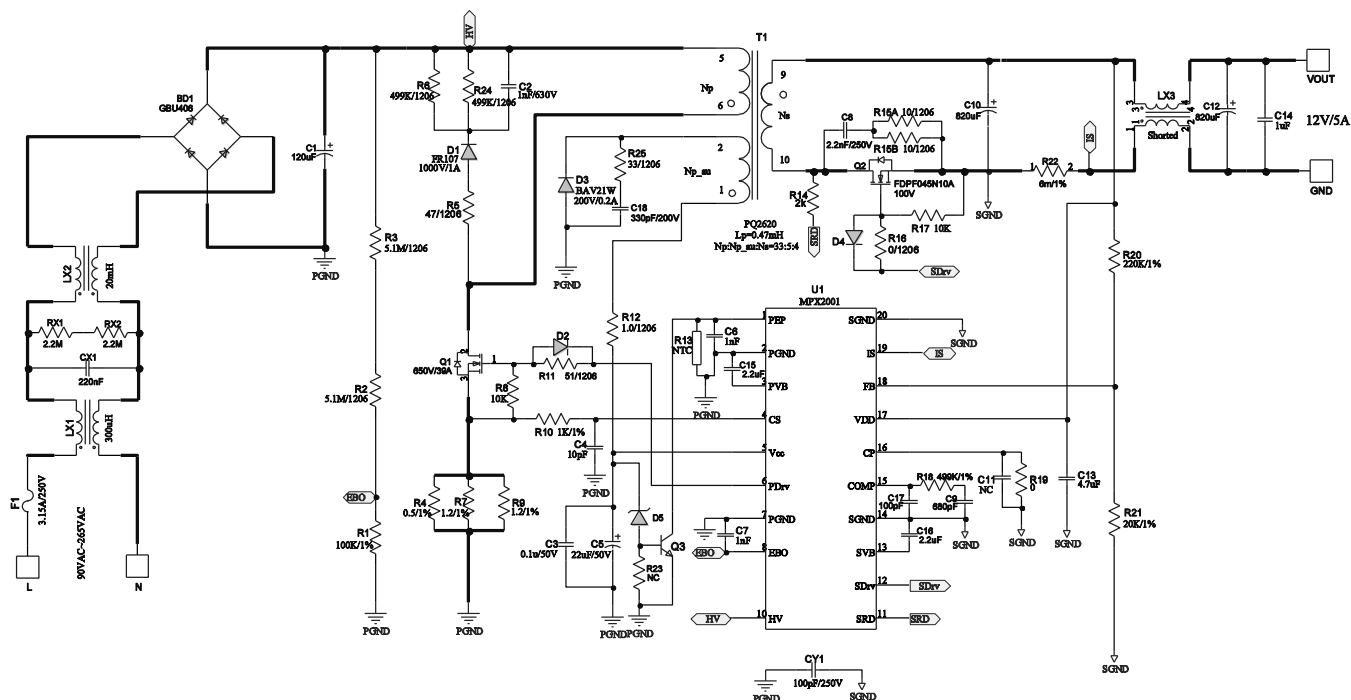
Figure 1—Schematic
