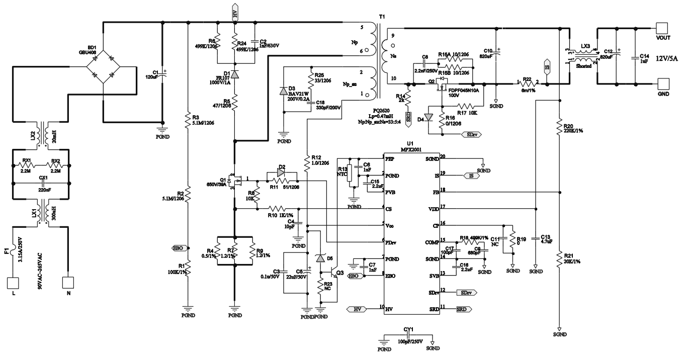
Figure 1—Schematic
