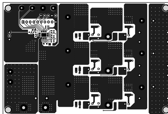
Figure 3: Top Layer
