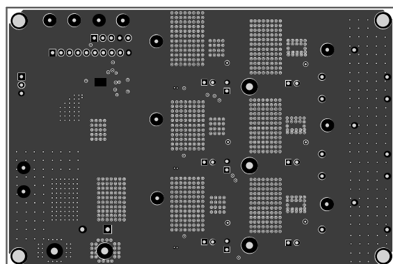
Figure 4: Mid-Layer 1
