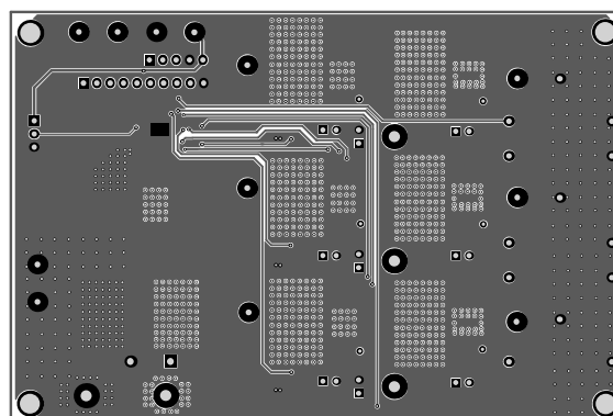
Figure 5: Mid-Layer 2
