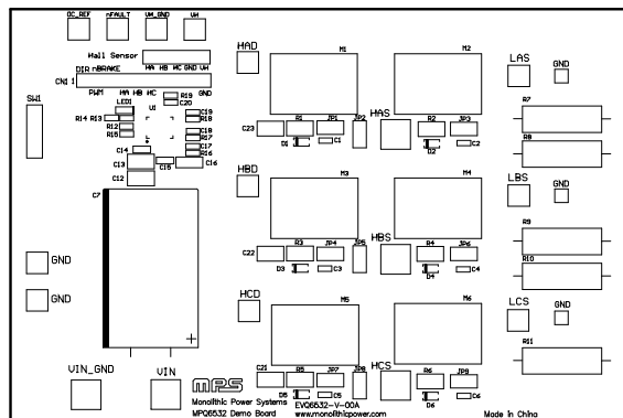
Figure 2: Top Silk
