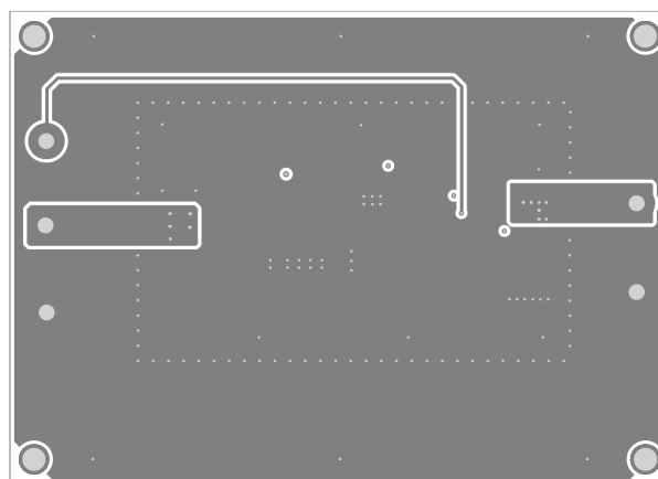
Figure 2—Inner2 Layer
