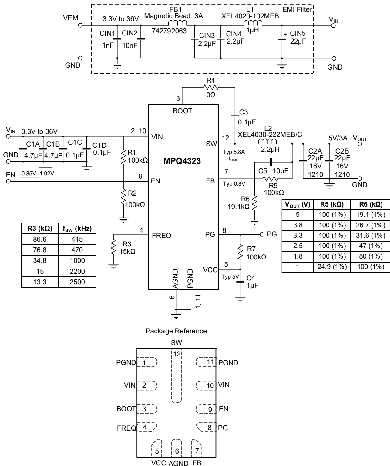
Figure 3: Evaluation Board Schematic
