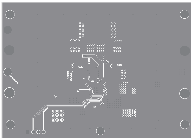
Figure 5: Middle Layer 3
