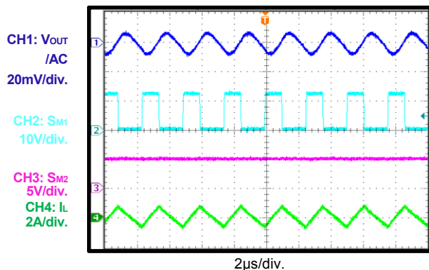
Steady state , V OUT =12V , BB_FSW=1 , Load=0A
