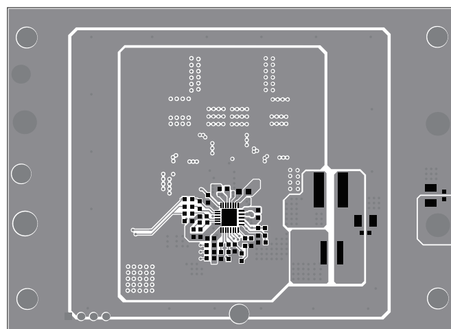
Figure 8: Bottom Layer
