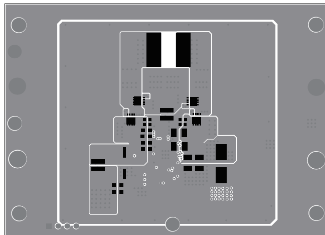
Figure 2: Top Layer
