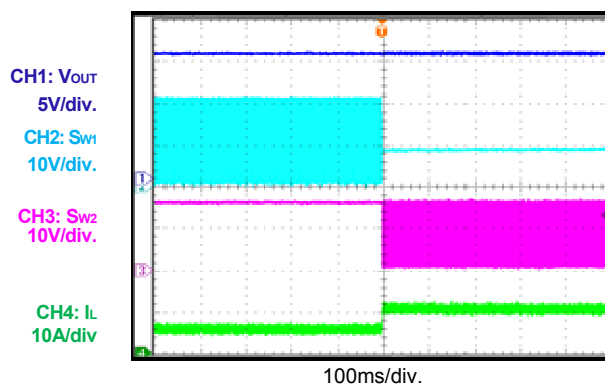
Input Voltage Transient, V_{IN}=20V to 9V , V_{OUT}=15V , Load= 5A
