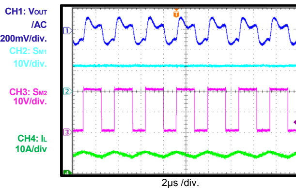
Steady state , V OUT =20V Load=5A
