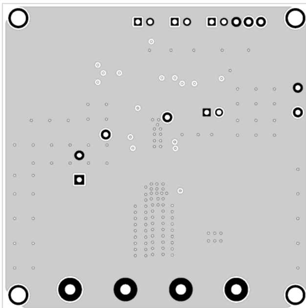
Figure 3: Inner 1 Layer & Inner 2 Layer
