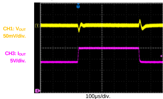
Load Transient@25% to 50% Load, 2.5A/µs
