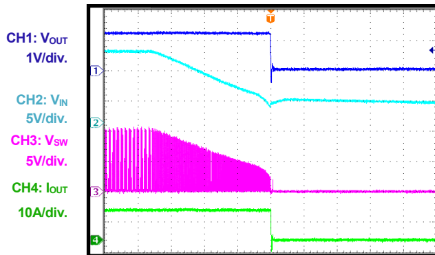
Vin Shutdown Through Input Voltage
