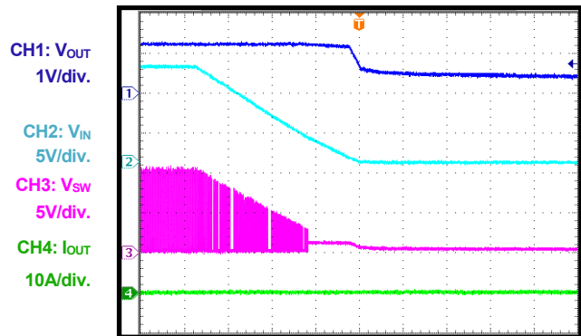
Vin Shutdown Through Input Voltage
