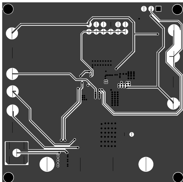
Figure 5-Inner2 Layer
