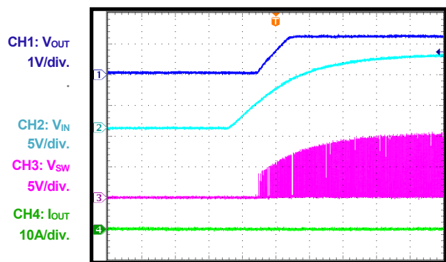
Vin Start-Up Through Input Voltage
