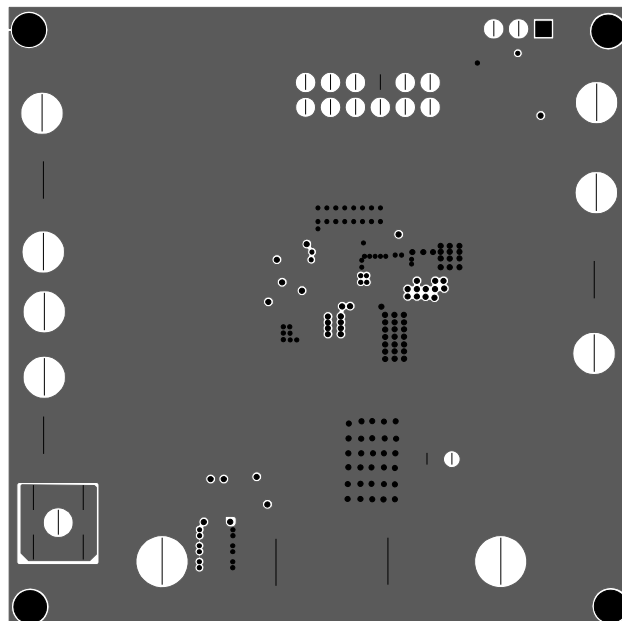
Figure 6-Inner3 Layer
