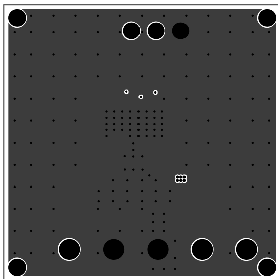
Figure 3—Inner1 Layer
