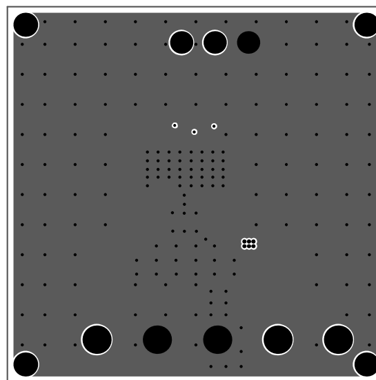
Figure 4—Inner2 Layer
