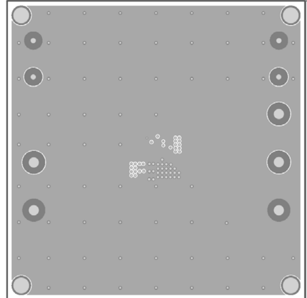
Figure 2-IN1 Layer
